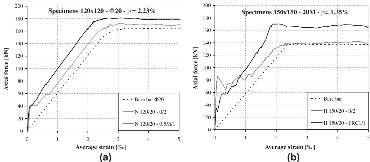
Fig. 3. Typical response of a NSRC and NSFRC (a) and HSRC and HSFRC tie elements (b).
