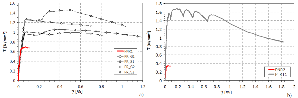
Figure 3. Shear stress-shear strain relationship for the panels tested: a) Panel built with mortar M10/UNI-EN 998-2; b) Panel built with mortar M2/UNI-EN 998-2
