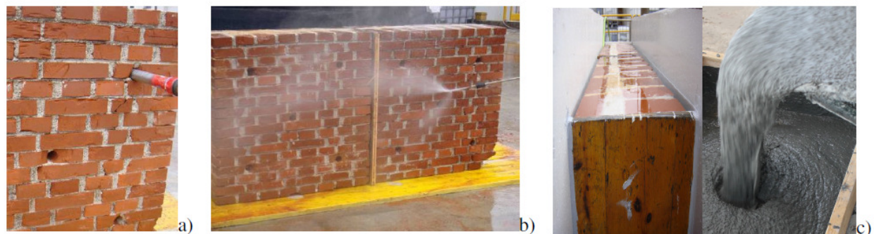
Figure 2. Application of the strengthening layer on the panel P_RT1: a) Execution of five through hole; b) Hydro cleaning of the surface; c) Realization of the moulds e casting
