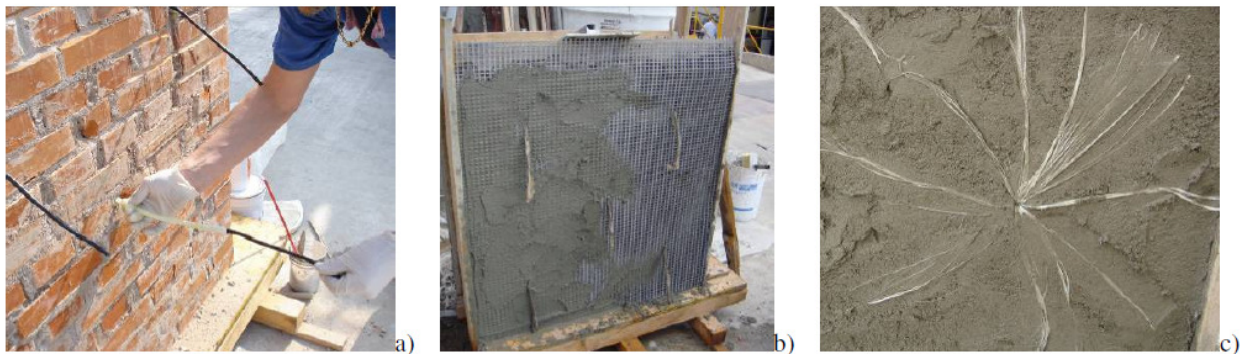
Figure 1. Application of the strengthening layer on the panel PR_G1: a) Insertion of the glass fiber wires; b) Positioning of the mesh; c) Anchoring of the connectors.
